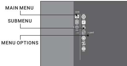
FIGURE 2-9. MAIN MENU
