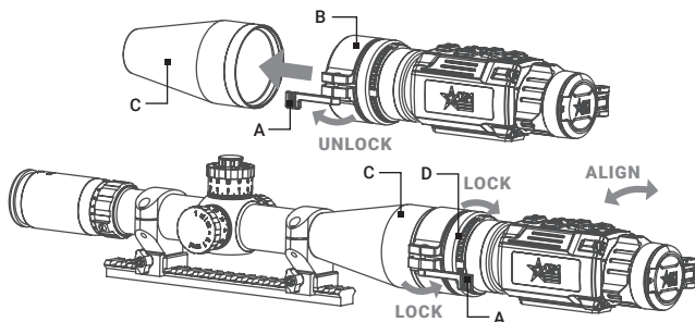
FIGURE 2-6. CLIP-ON INSTALLATION
