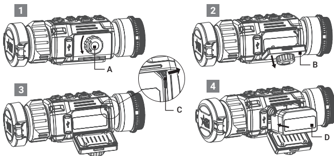
FIGURE 2-1. BATTERY INSTALLATION
