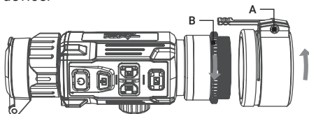
FIGURE 2-5. FRONT Q-R ADAPTER INSTALLATION
