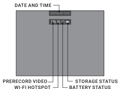
FIGURE 2-3. ON-SCREEN DISPLAY
