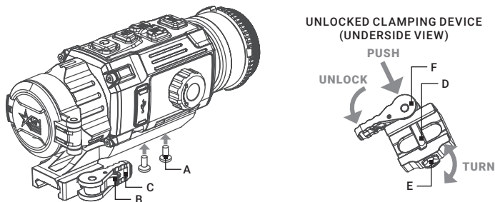
FIGURE 2-8. MOUNT
