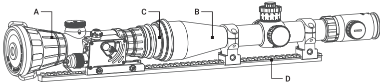
FIGURE 2-3. COMANCHE-40ER ON A PICATINNY RAIL IN FRONT OF A DAY SCOPE
