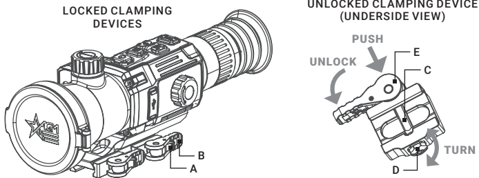
FIGURE 2-5. MOUNT
